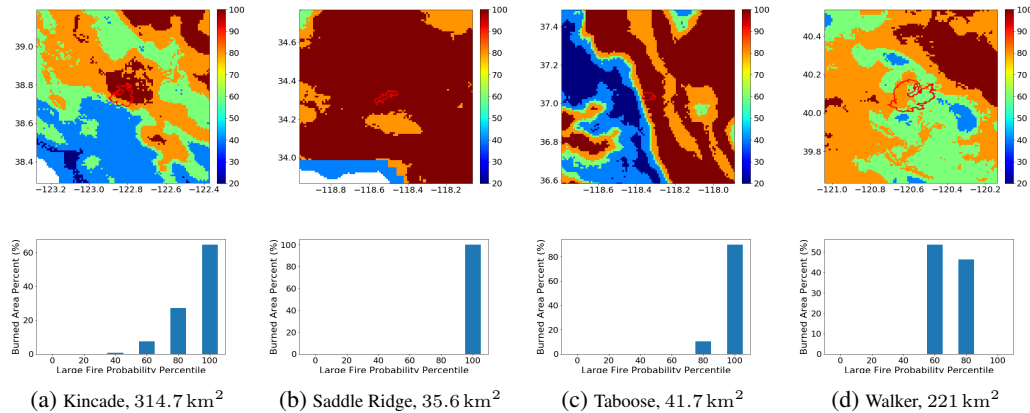
Figure 4: Four severe fire incidents in 2019 (a-d) Kincade, Saddle Ridge, Taboose and Walker. Top: LFP percentile maps overlaid with the perimeter of the fire incident in the first two days. Bottom: summaries of burned pixels percentage of each percentile bin
