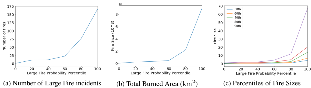
Figure 3: The relationships between LFP percentiles and historical fire activity: (a) counts of fire incidents with fire size larger than 4 \text{ km}^2 , (b) cumulative burned area in each percentile bin and (c) percentiles of individual fire size from 2012-2016.
