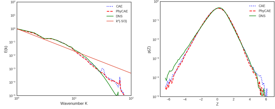
(a) Kolmogorov Energy Spectra: CAE and PhyCAE vs DNS (b) PDFs of velocity gradient: CAE and PhyCAE vs DNS
